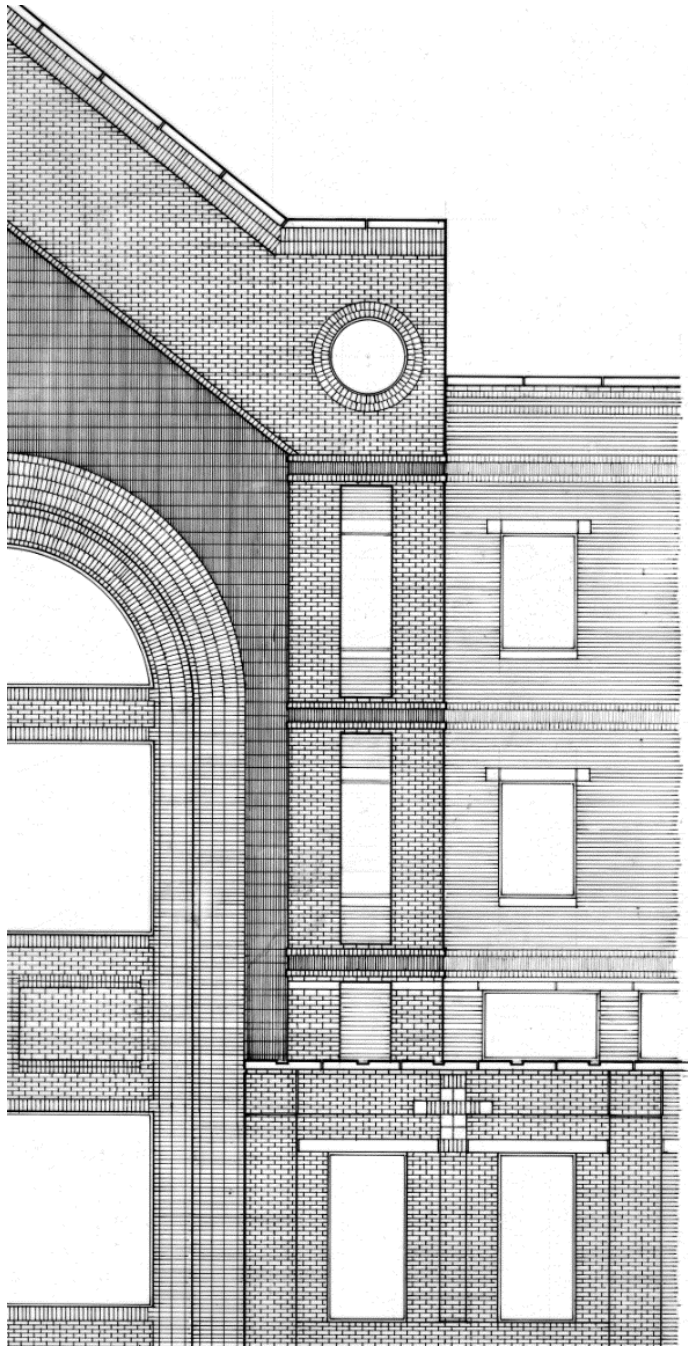
Goldring-Woldenberg Hall, A.B. Freeman School of Business, Tulane University. 1985. Concordia Architects. Ink on mylar.
