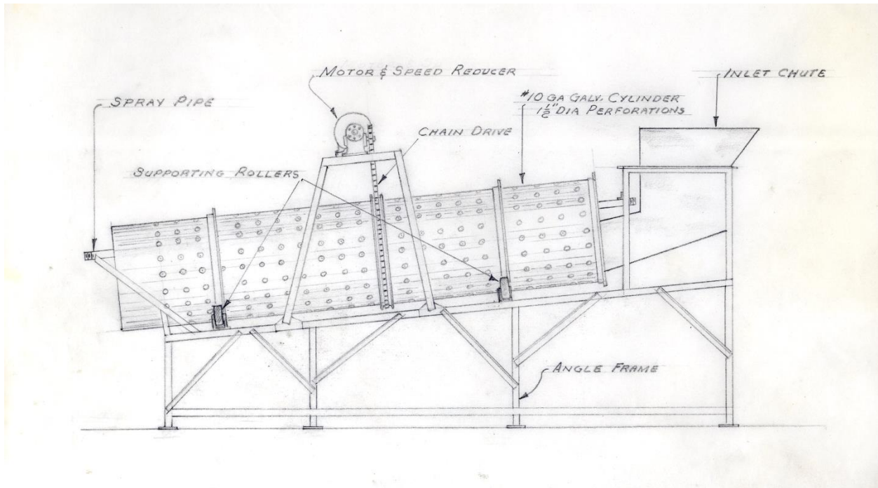
Blattmann Sheet Metal Works, Inc. Design for an oyster washer. Client unidentified. 1952. Pencil on small sheet of tracing paper.
