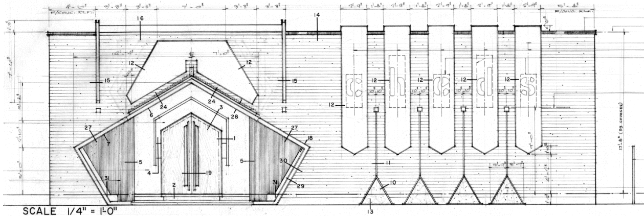
Ched's Lounge, Canal Street and North Claiborne Avenue, New Orleans, La. 1962. Robert L. Schenker, architect. Ink on tracing paper.
