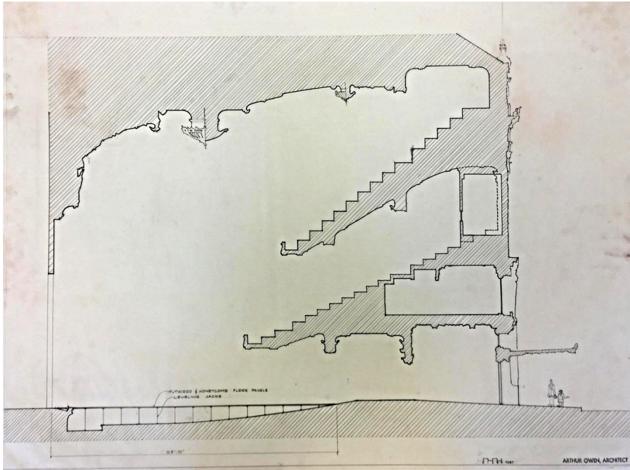
Profile of Orpheum Theater, New Orleans, LA. 1980. Arthur M. Owen, architect. Ink and pencil on tracing paper.
