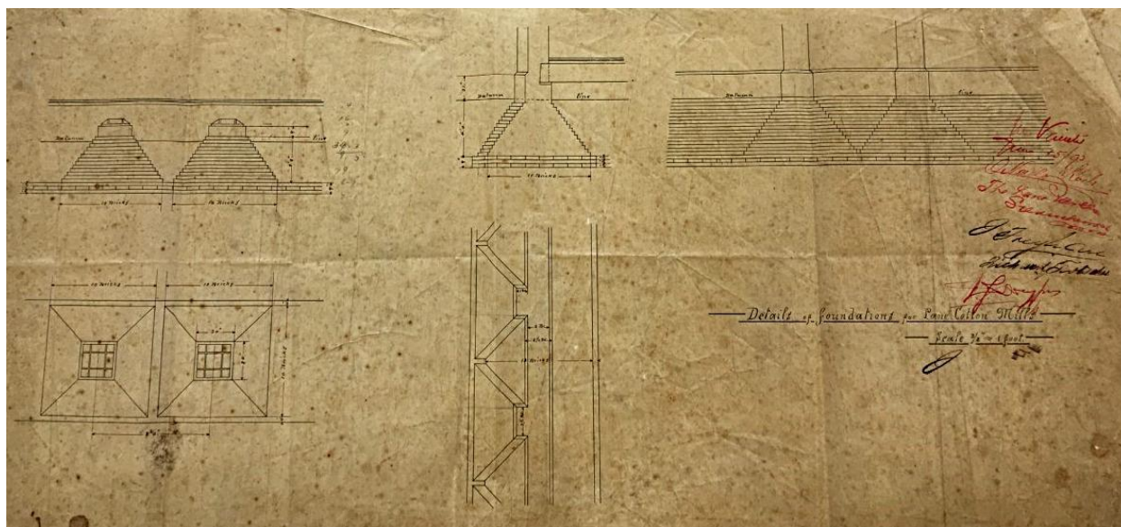
Lane Cotton Mills, detail of foundations, New Orleans, LA. 1892. O'Neil and Koch, architects. Ink and colored ink on paper.
