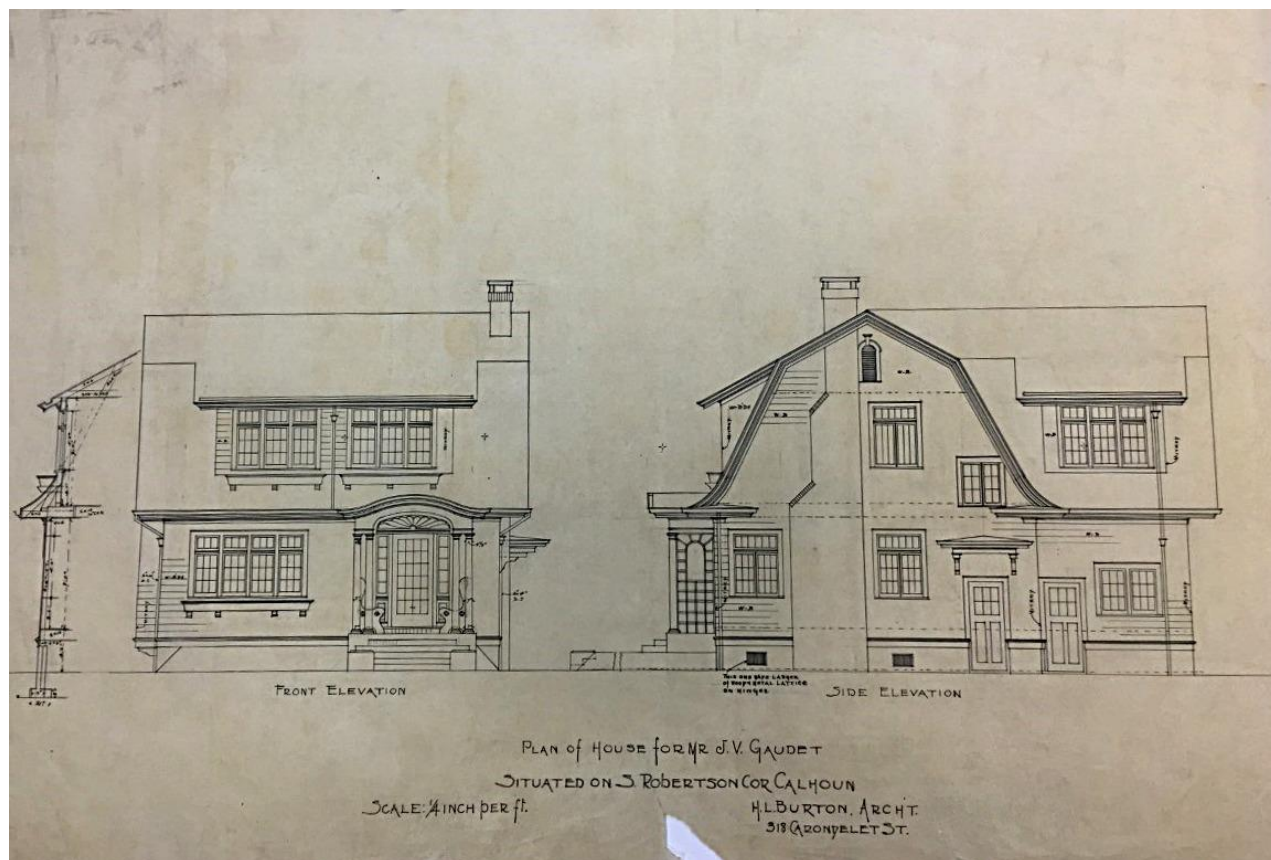
James Gaudet Residence, South Robertson and Calhoun Streets, New Orleans, LA. Undated. H.L. Burton, architect. Pencil on tracing paper.
