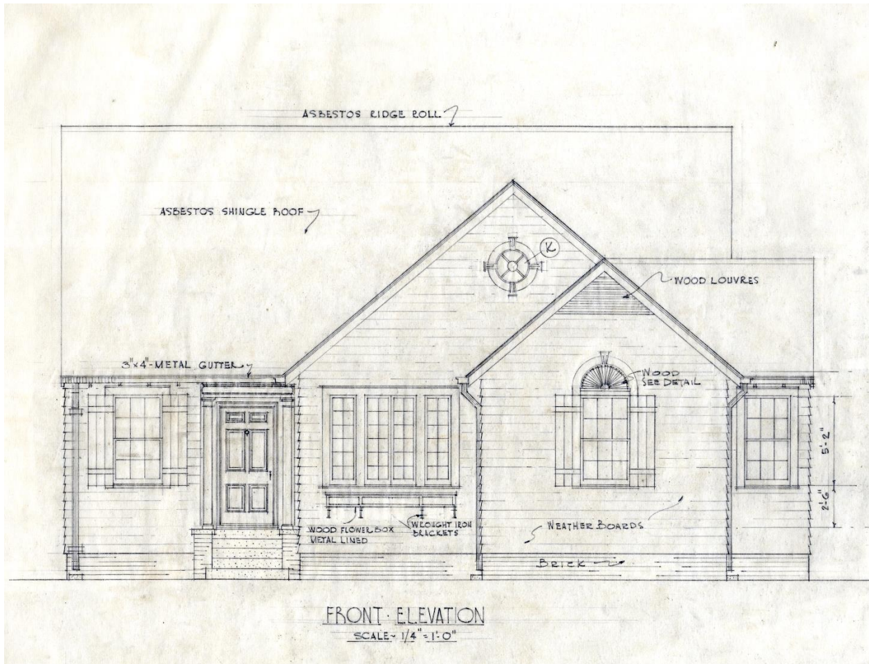
Lake Vista, New Orleans, LA. Mr. and Mrs. G.H. Willian Residence. 1946. Ammen and Lockett, architects. Pencil on tracing paper.
