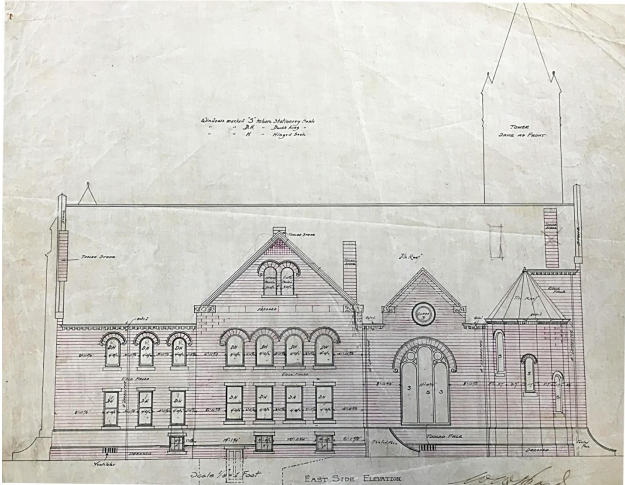
First Baptist Church, 3436 St. Charles Avenue, New Orleans, LA. Undated. F.J. MacDonnell, architect. Ink and red ink, and pencil on linen.
