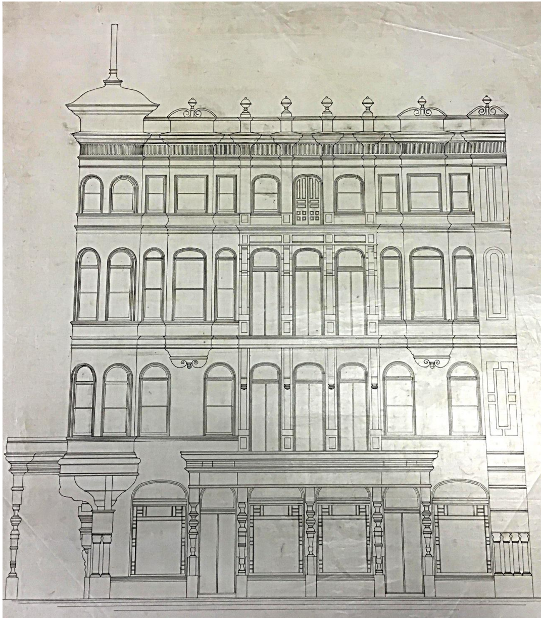
Pickwick Club, alterations to exterior. 1894. Toledano and Reusch, architects. Ink on linen.
